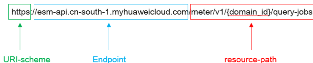
Figure 3-1 Example URI
